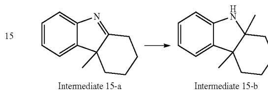
Reaction Scheme 16
