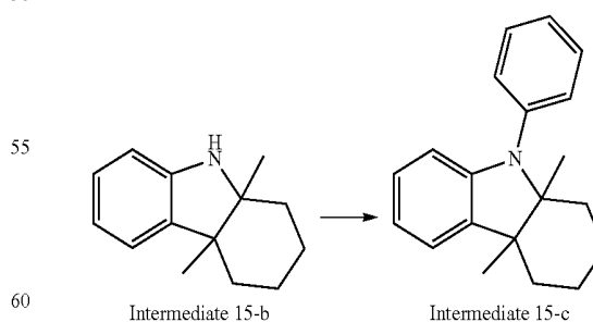
Reaction Scheme 17
