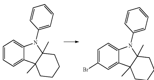
Reaction Scheme 18
