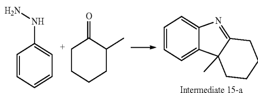
Reaction Scheme 15
